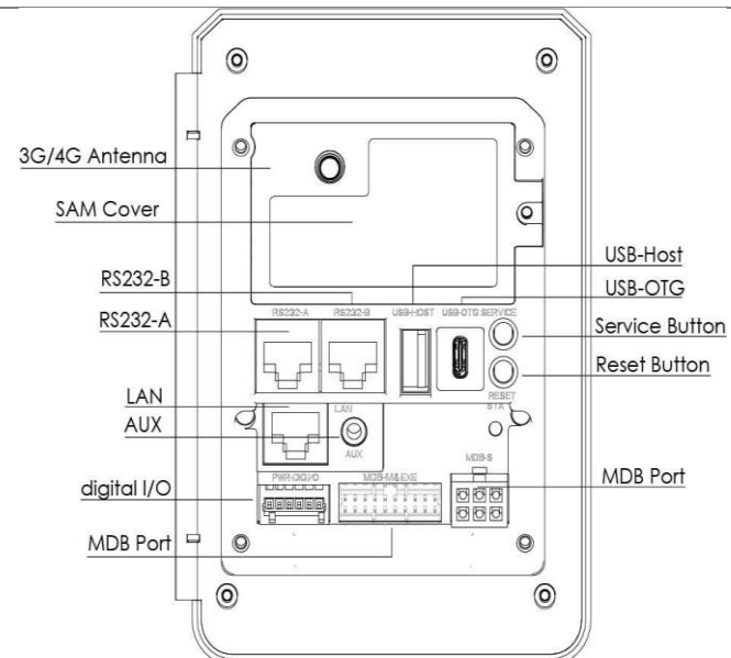
Figure 2: PAX IM30 Back side
