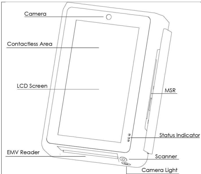
Figure 1: PAX IM30 Front side
